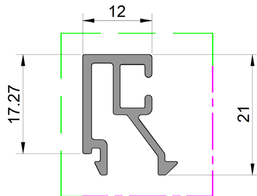
Bead for 36mm Triple Glazed
